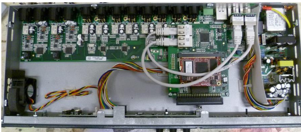
Internal view of version with Dante card fitted
